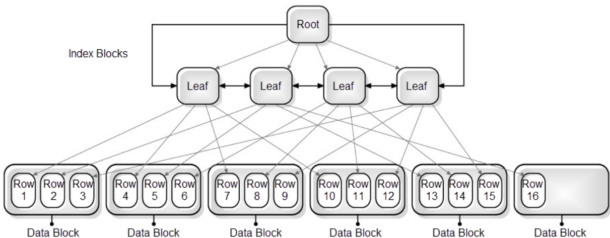
Figure 2 Index with bad clustering factor (high = number of rows)
