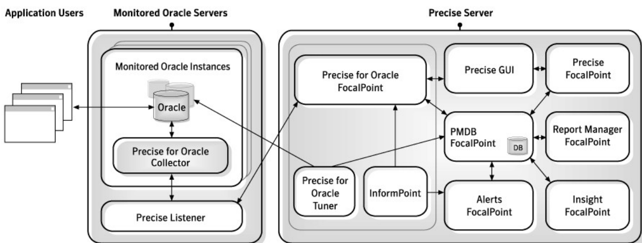
Figure 1 Precise for Oracle architecture
