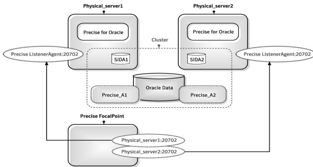
Figure B-3 Parallel partitions configuration in an Oracle application
