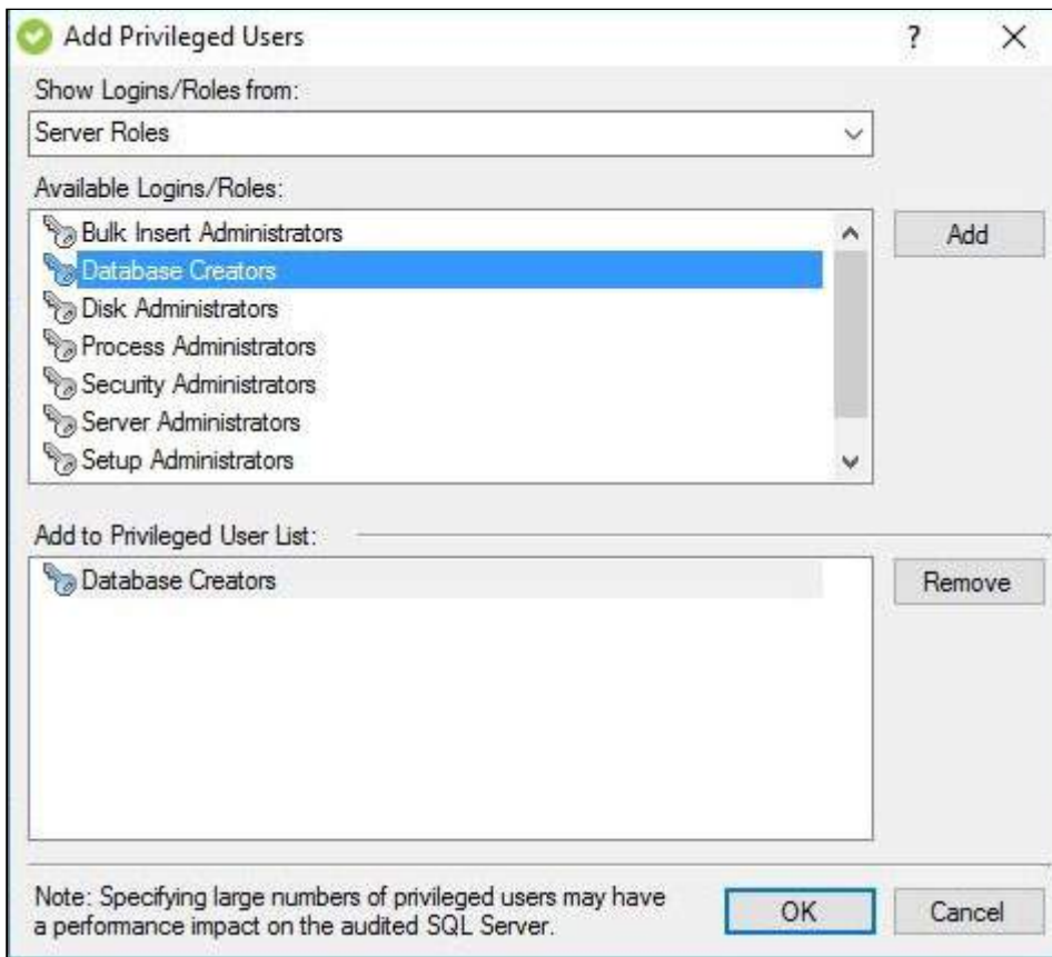
Configuration wizard Add Audited Database - Privileged Users Audited Activity window
